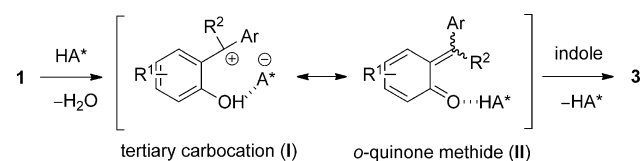
Scheme 2. Proposed mechanism.
